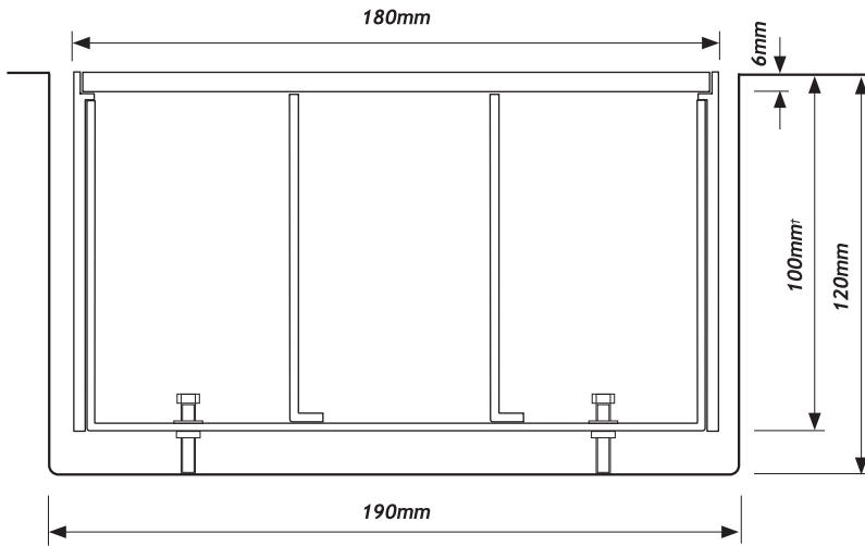
Triple Compartment Floor Channel - 180x100/3 shown
