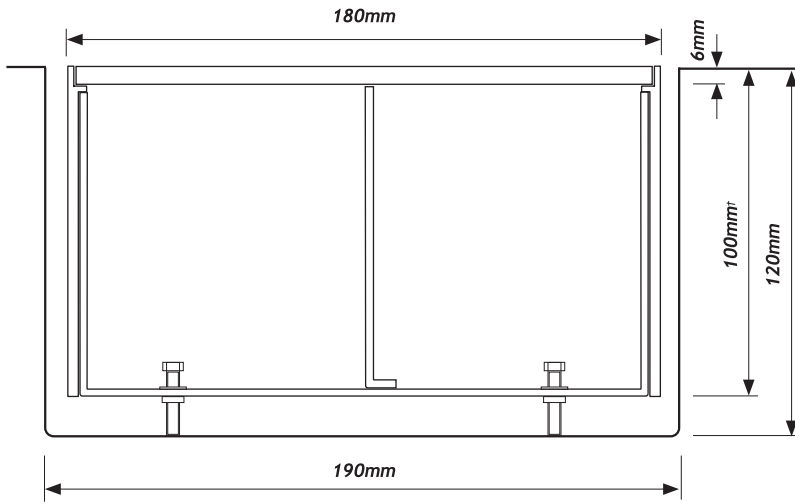
Double Compartment Floor Channel - 180x100/2 shown
